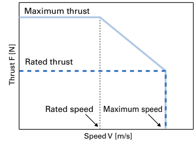
Thrust-Speed Characteristics
